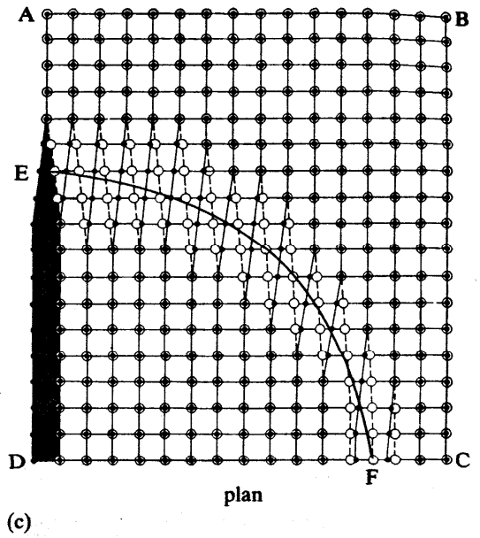
Figure 2.56 (a) Slip part way across the plane ABCD in block model. (b) and (c) show atomic model. In (c) atoms below the slip plane are represented by a dot. Those above are represented by a circle. A circle with a dot indicates atoms in register
